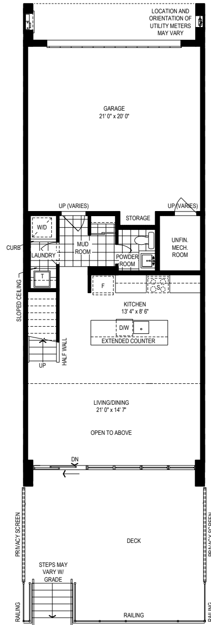
GROUND LEVEL
