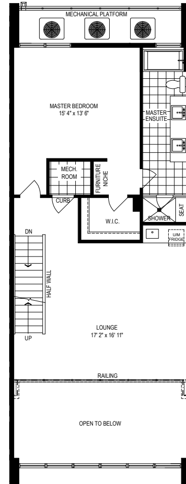
SECOND LEVEL
