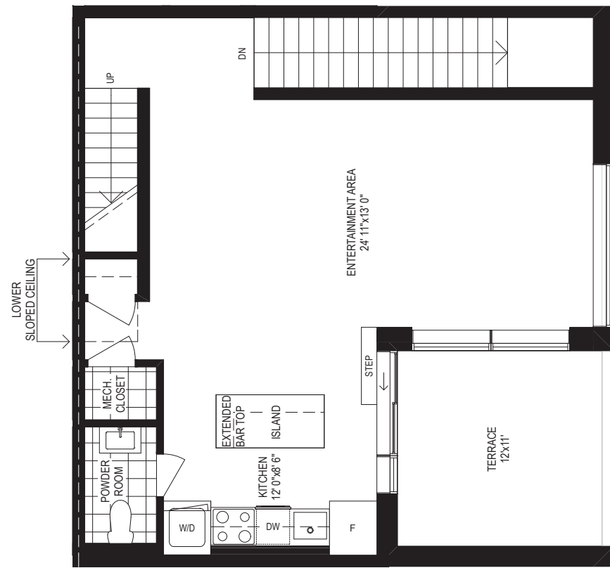
LEVEL 2
