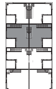
SECOND LEVEL
