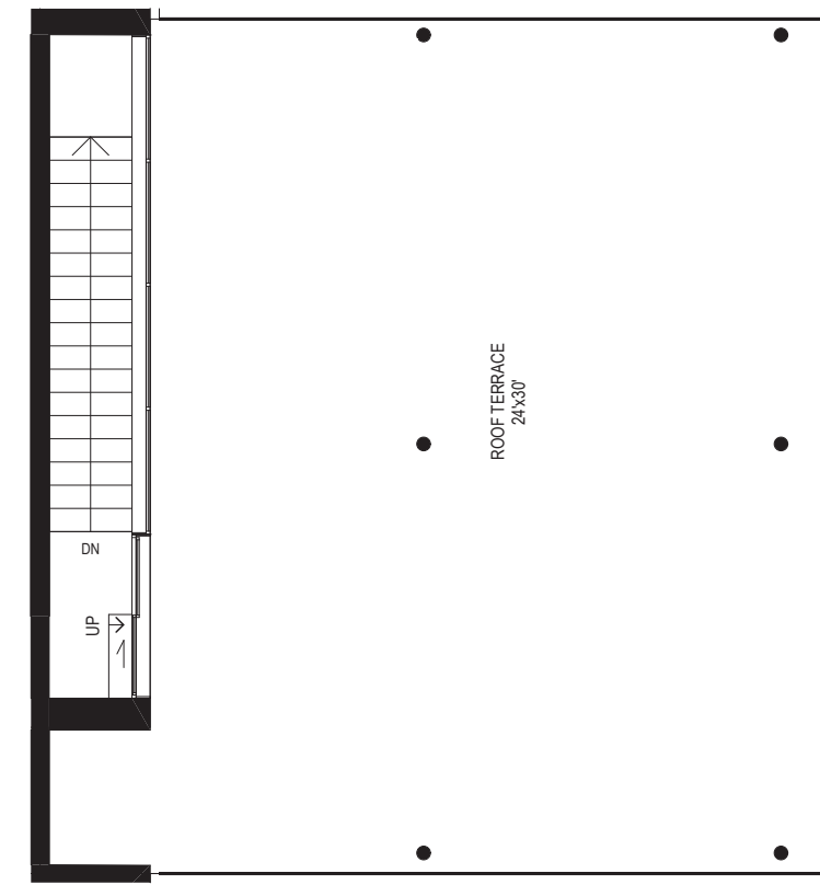
ROOF LEVEL
