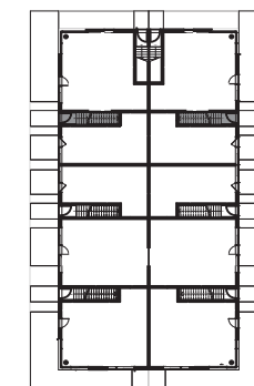
GROUND LEVEL
