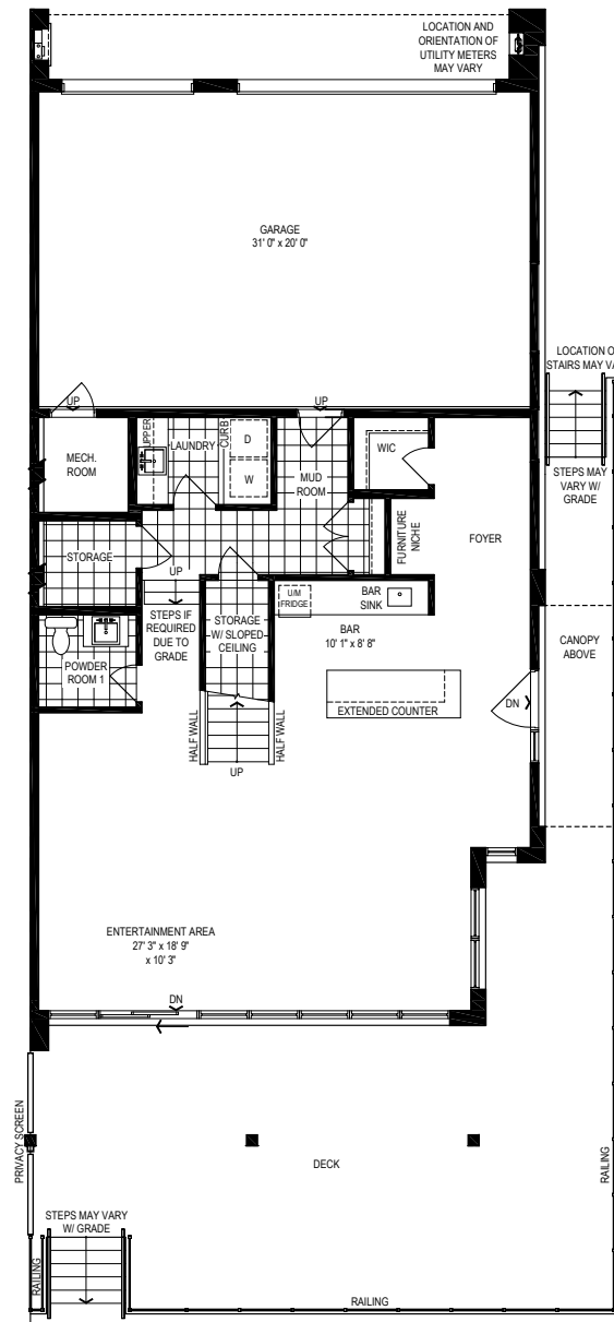
GROUND LEVEL
