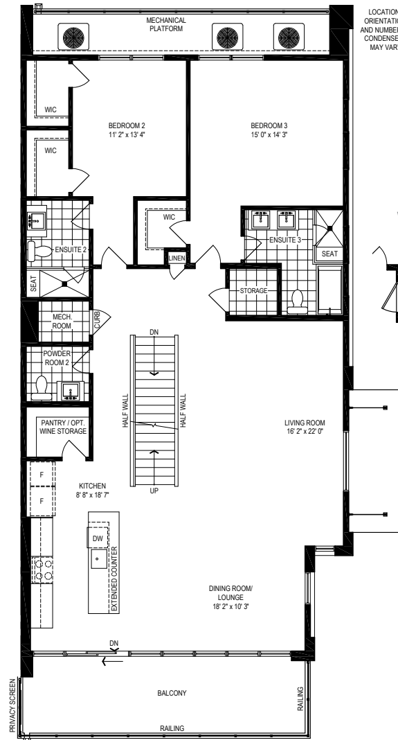
SECOND LEVEL
