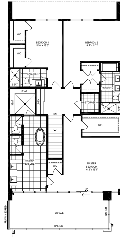
THIRD LEVEL
