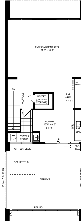
THIRD LEVEL OPT. 2 W/ ELEVATOR
